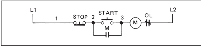
Figure 1 Three Wire Control Giving Low Voltage Protection Using Single Two Button Station
