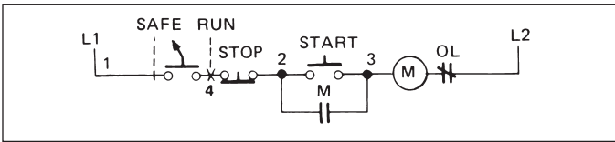
Figure 3 Three Wire Control Giving Low Voltage Protection with Safe-Run Selector Switch
