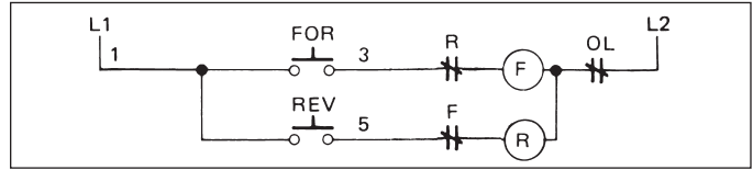
Figure 8 Two Wire Control for Reversing Jogging Using Single Two Button Station
